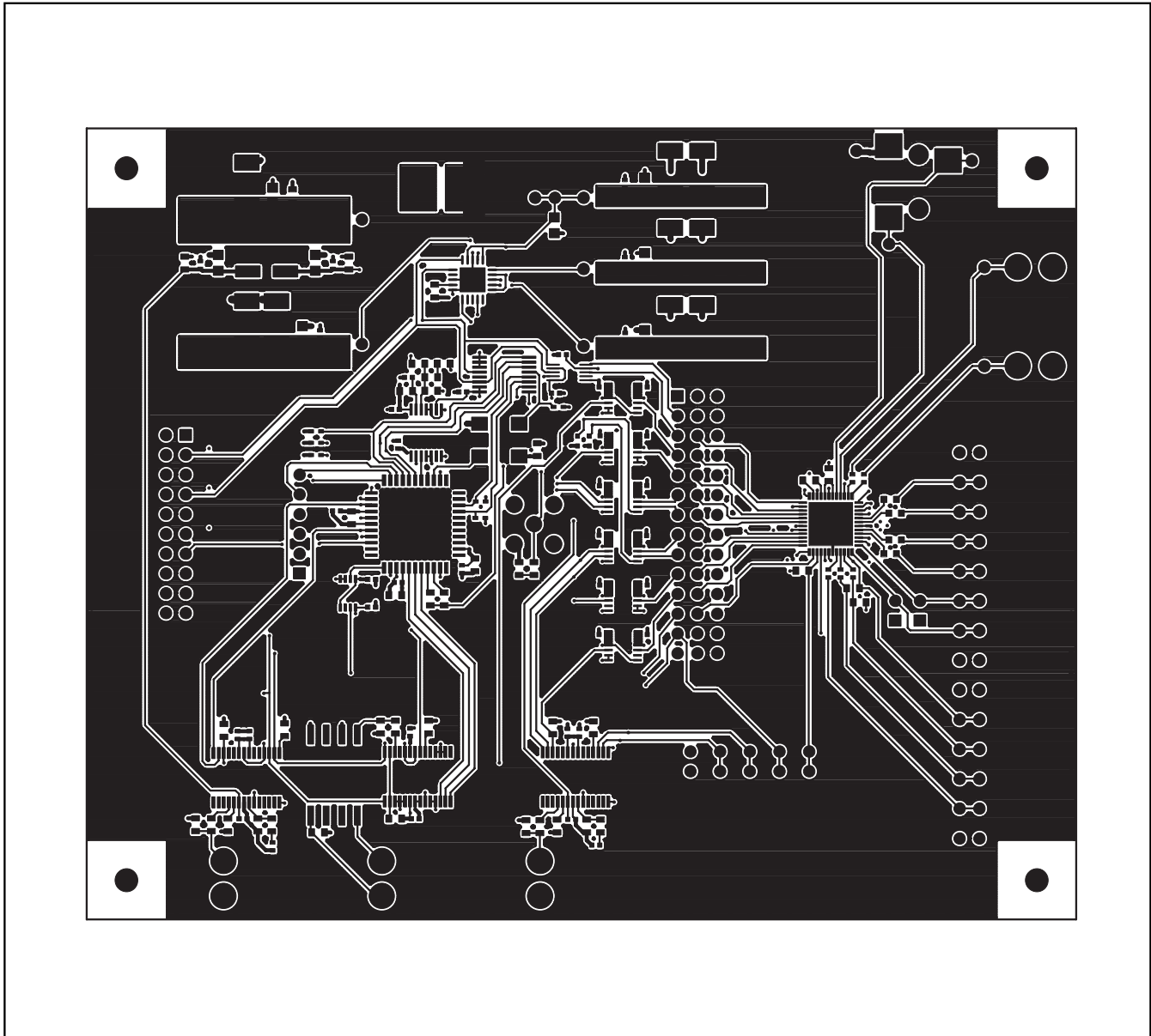
Figure 24. MAX9851 EV Kit PCB Layout—Component Side
