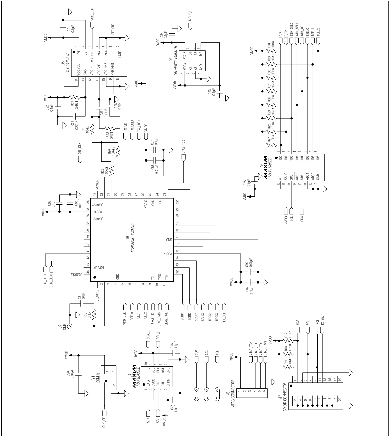
Figure 21. MAX9851 EV Kit Schematic (Sheet 2 of 3)
