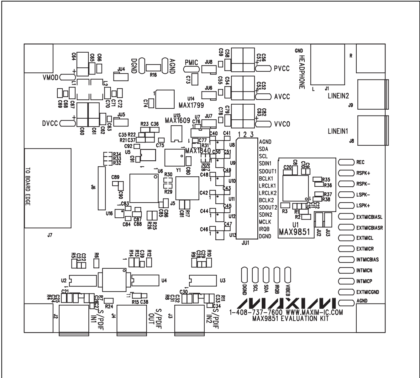
Figure 23. MAX9851 EV Kit Component Placement Guide—Component Side
