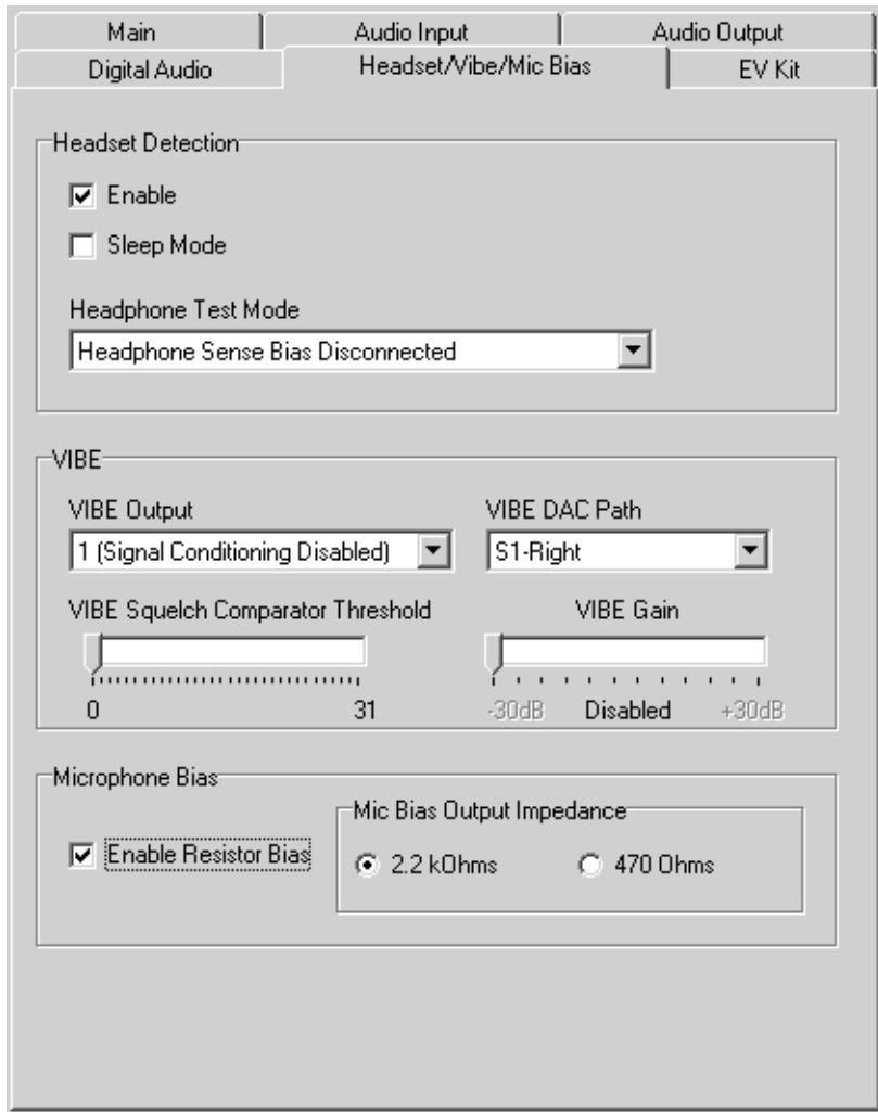
Figure 13. MAX9851 EV Kit Headset/Vibe/Mic Bias Control Page
