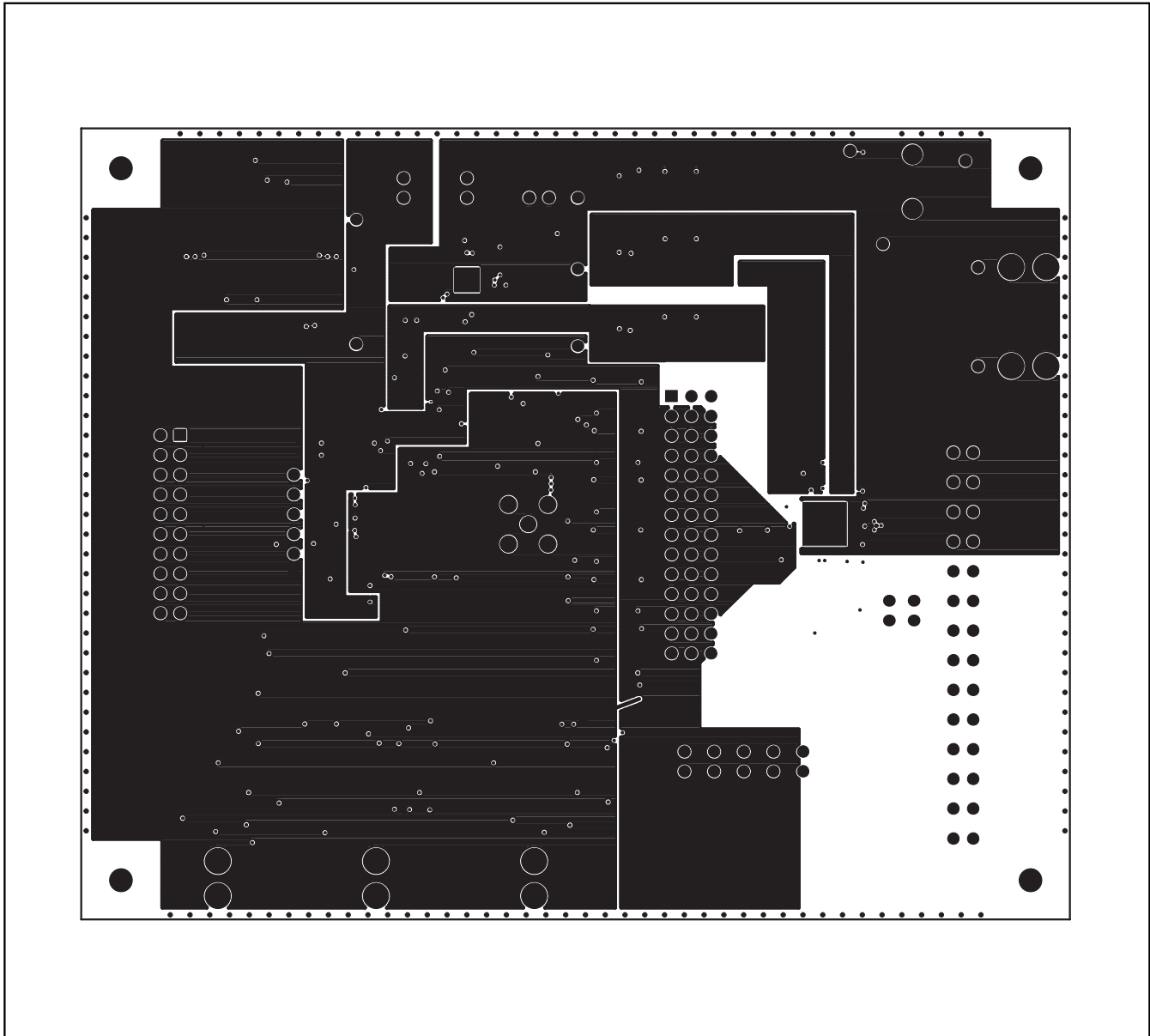
Figure 26. MAX9851 EV Kit PCB Layout—Inner Layer 3
