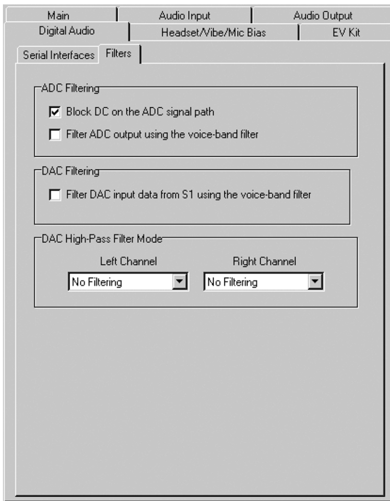
Figure 12. MAX9851 EV Kit Digital Audio—Filter Control Page
