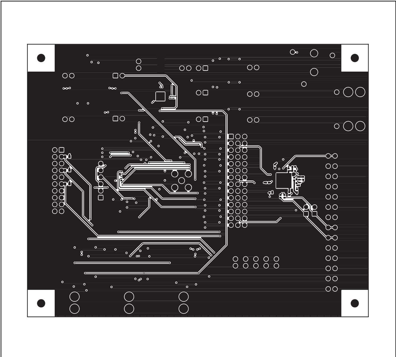
Figure 27. MAX9851 EV Kit PCB Layout—Solder Side
