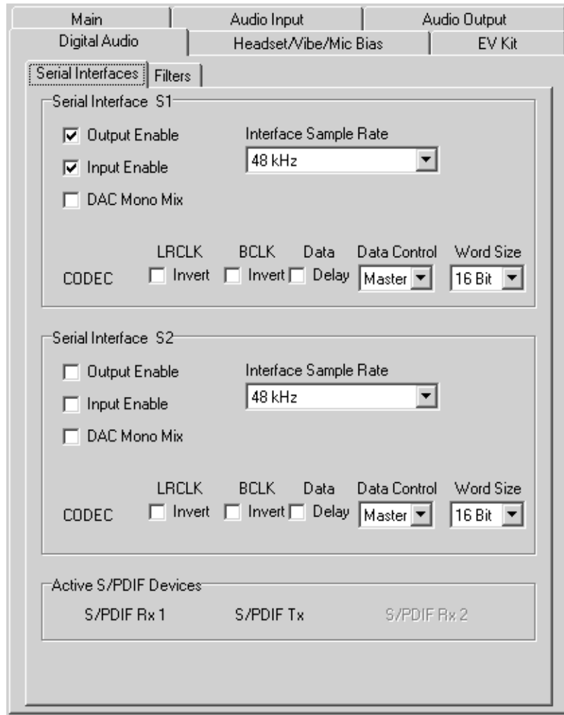
Figure 11. MAX9851 EV Kit Digital Audio—Serial Interface Control Page
