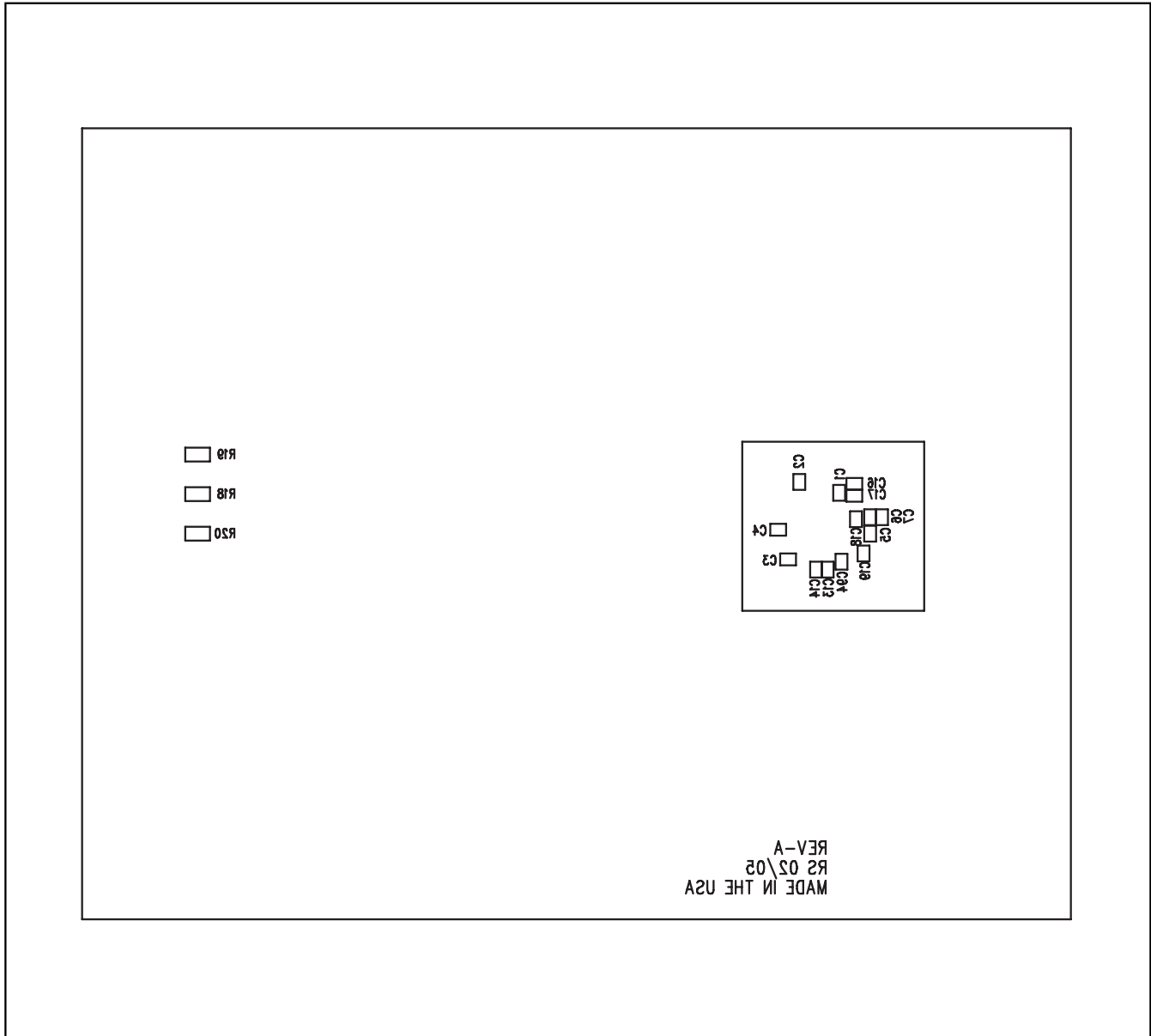
Figure 28. MAX9851 EV Kit Component Placement Guide—Solder Side
