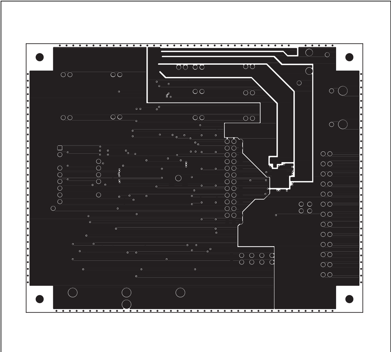
Figure 25. MAX9851 EV Kit PCB Layout—Inner Layer 2
